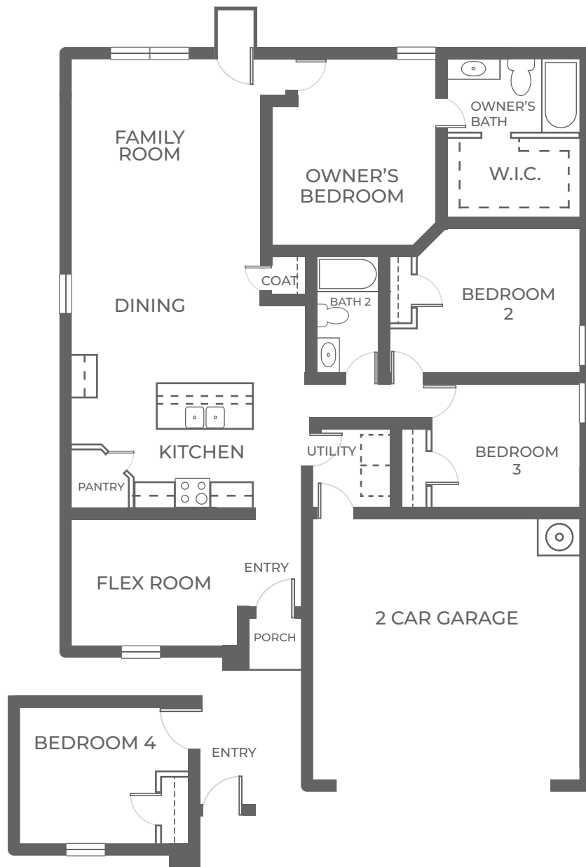
BEDROOM 4 OPTION
